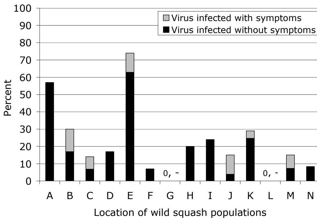
Figure 2.2. Prevalence of virus in all plants (black bars) and prevalence of virus in plants exhibiting virus symptoms (gray bars) in wild squash populations in the south-central USA in 2004. Site abbreviations along x-axis are A: Alpena, AR; B: Berryville, AR; C: Bigelow, AR; D: Bradley, AR; E: Canale, AR; F: Cozahome, AR; G: Gilbert, AR; H: Moreland, LA; I: Woodworth, LA; J: Fidler, MS; K: Eagle Lake, MS; L: Simcoe, MO; M: Washburn, MO; N: Park Hill, OK
